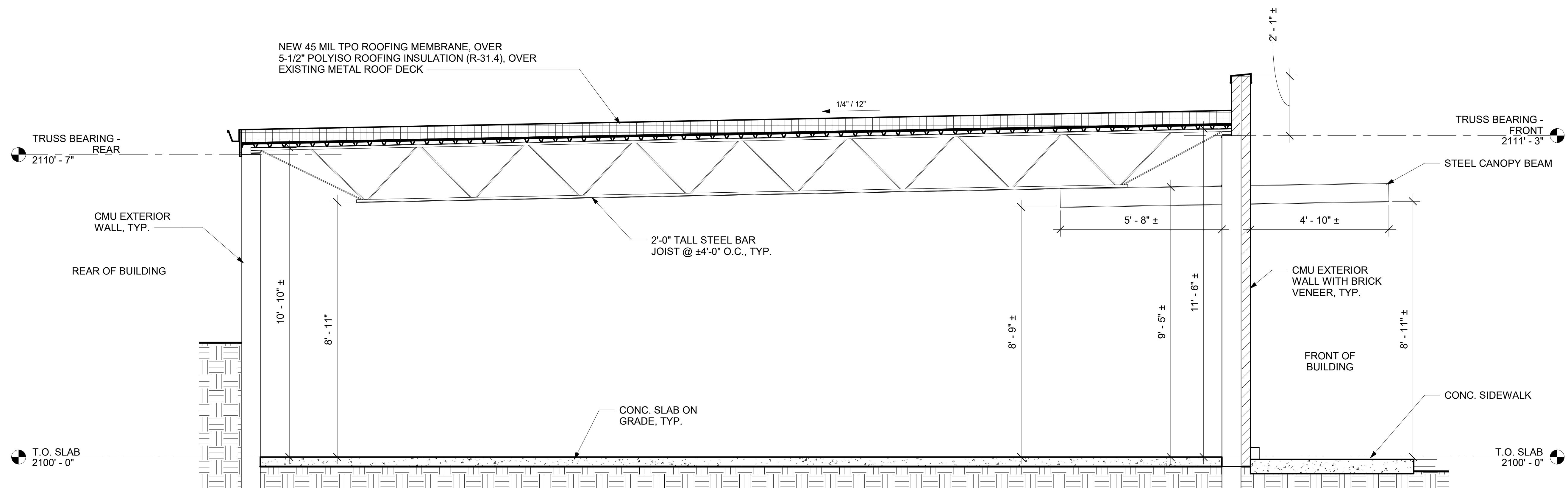
1 EXISTING BUILDING SECTION - NORTH SOUTH A301 1/2" = 1'-0"
